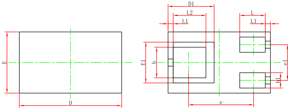
BOTTOM VIEW
