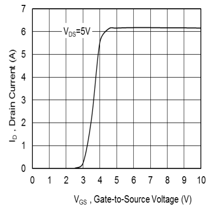
Fig.11 Transfer Characteristics
