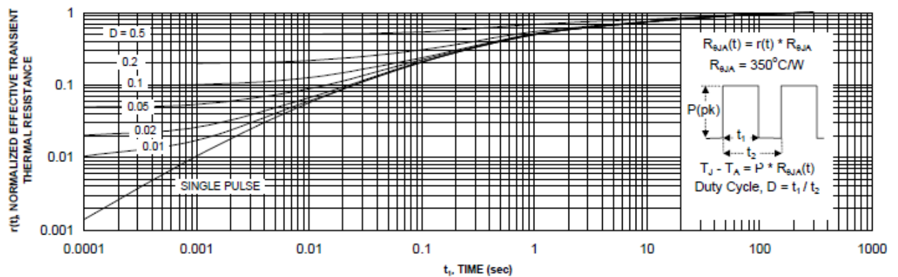
Transient Thermal Response Curve, Junction to Ambient
