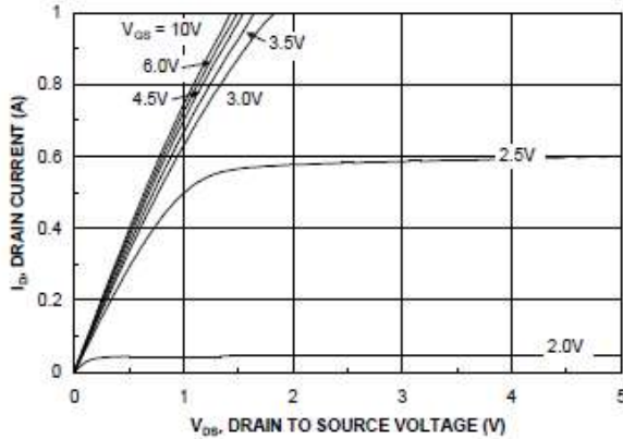
On-Region Characteristics
