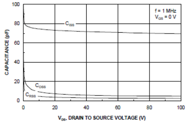
Capacitance Characteristics
