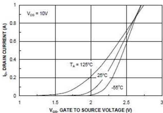
Transfer Characteristics
