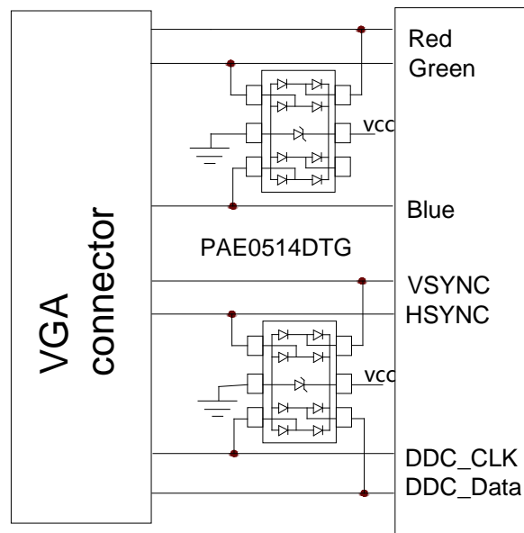
ESD protection for VGA port
