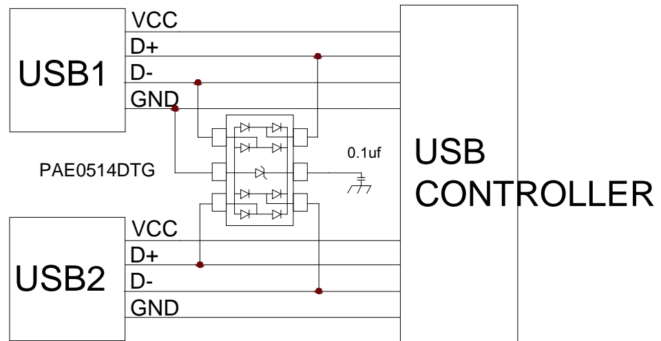
ESD protection for USB port
