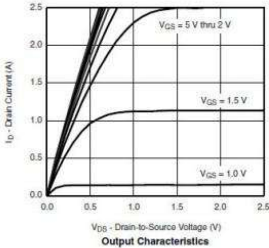
Output Characteristics
